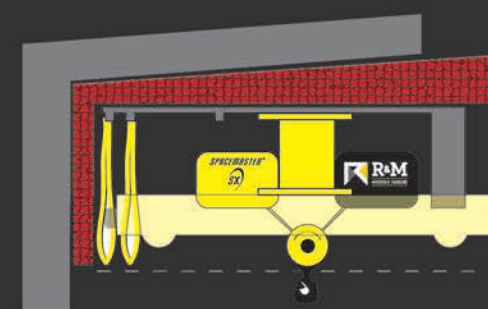
Figure 1. C-track Festoon
